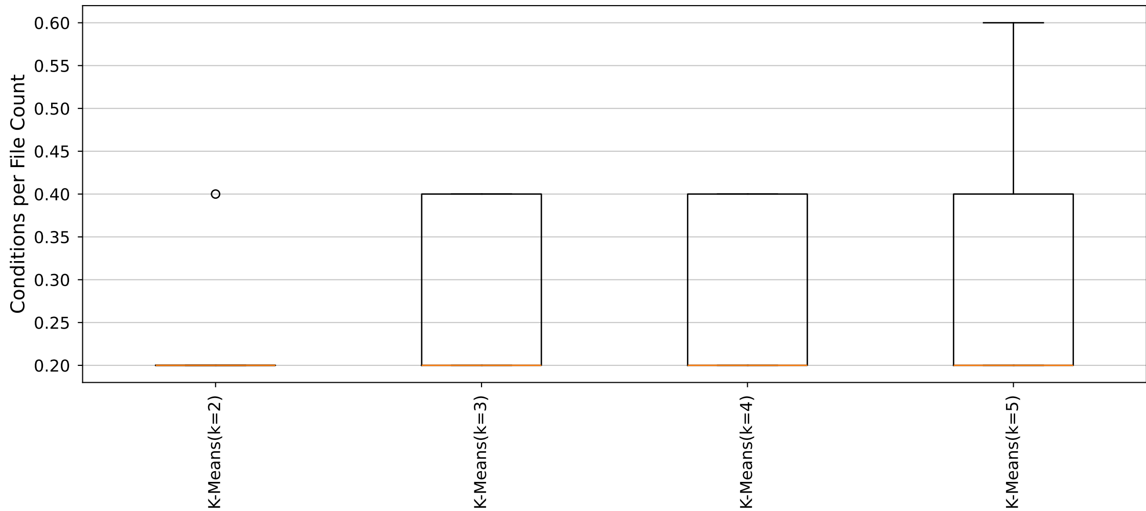
YARA Rules Conditions per File Count Distribution (Cluster37_Size5 dataset)
